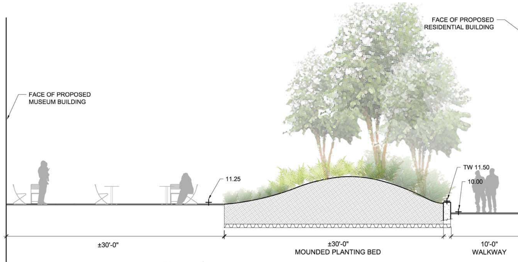
COURTYARD SECTION A-A
